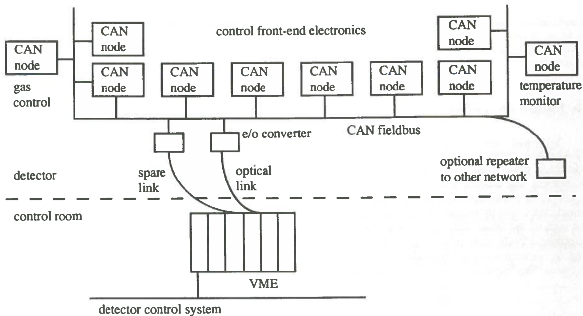
Fig. 3 Detector front-end control with a CANDIDE fieldbus system.
