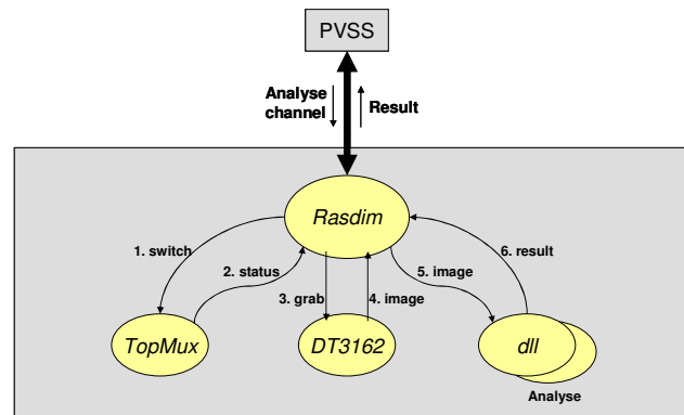
Figure 5: Rasdim control flow
