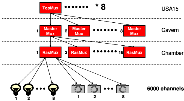
Figure 4: Multiplexer scheme
