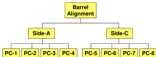
Figure 6: Barrel Alignment FSM hierarchy
